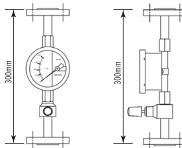
Model: MF200E-R
