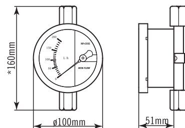
Model: MF200E-S
