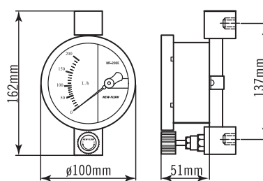
Model: MF200E-B
