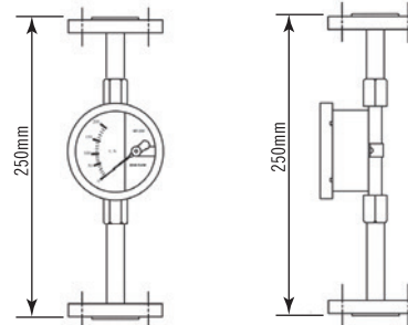
Model: MF200E-T
